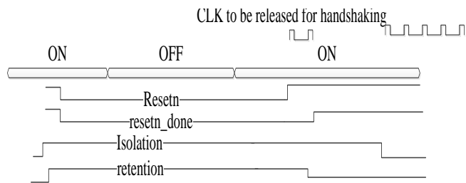
Figure 2 Reset handshaking
